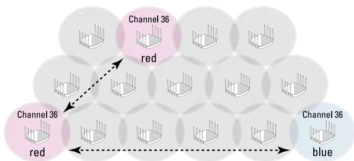
FIGURE 4-3: BSS color.
