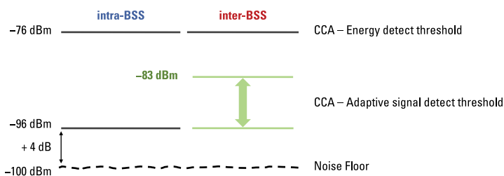
FIGURE 4-4: Spatial reuse operation - Adaptive CCA
